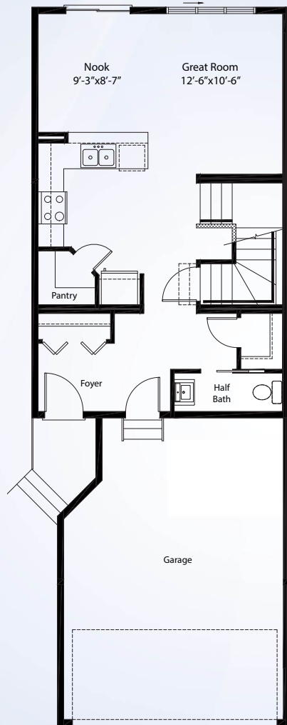
Main Floor | 640 Sq. Ft.
